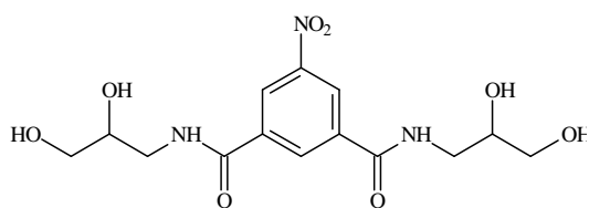
N,N'-Bis(2,3-dihydroxypropyl)-5-nitro-isophthalamide
