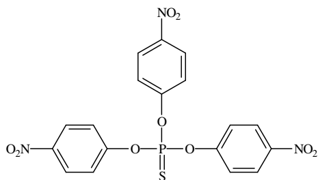
Tris-(4-nitrophenyl)-thiophosphate
