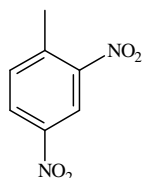
2,4-Dinitrotoluene
