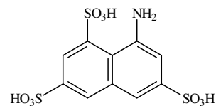
Amino-T-acid
