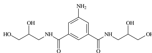
N,N'-Bis(2,3-dihydroxypropyl)-5-amino-isophthalamide
