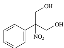
2-Nitro-2-Phenylpropane-1,3-diol
