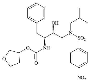
(3S)-Tetrahydro-3-furyl-N-[(1S,2R)-1-benzyl-2-hydroxy-3-(N-isobutyl-4-nitrobenzenesulfonamido)propyl]carbamate
