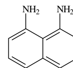
1,8-Diaminonaphtalene
