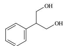
2-Phenylpropane-1,3-diol
