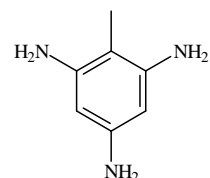
2,4,6-Triaminotoluene
