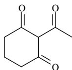
2-Acetylcyclohexane-1,3-dione
